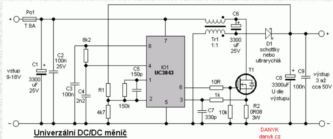
Schematic diagram of the universal DC / DC converter.
